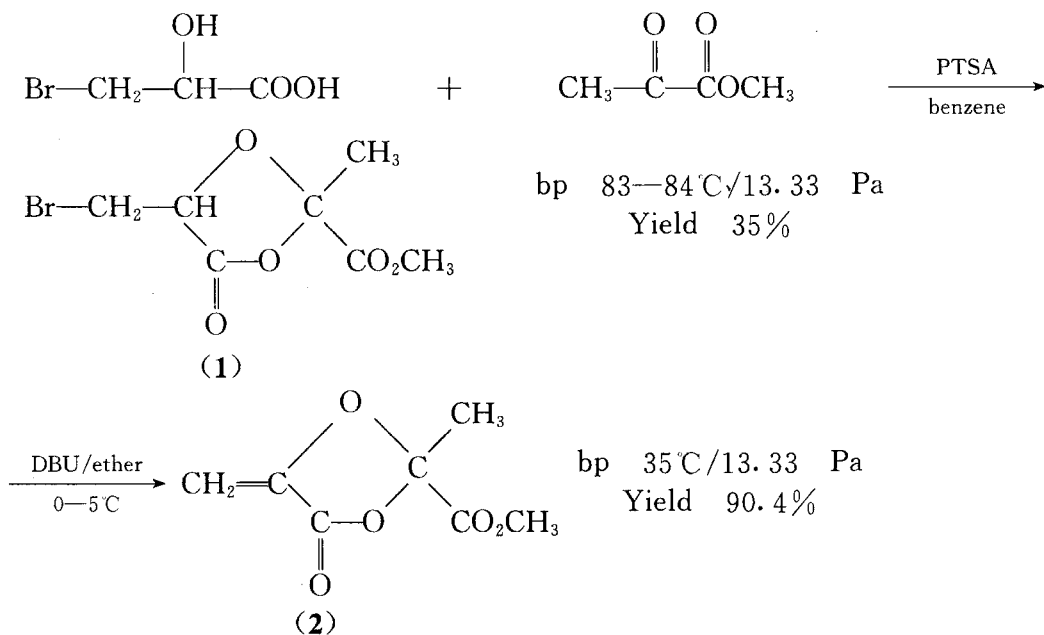
Scheme I Synthesis of Monomer
