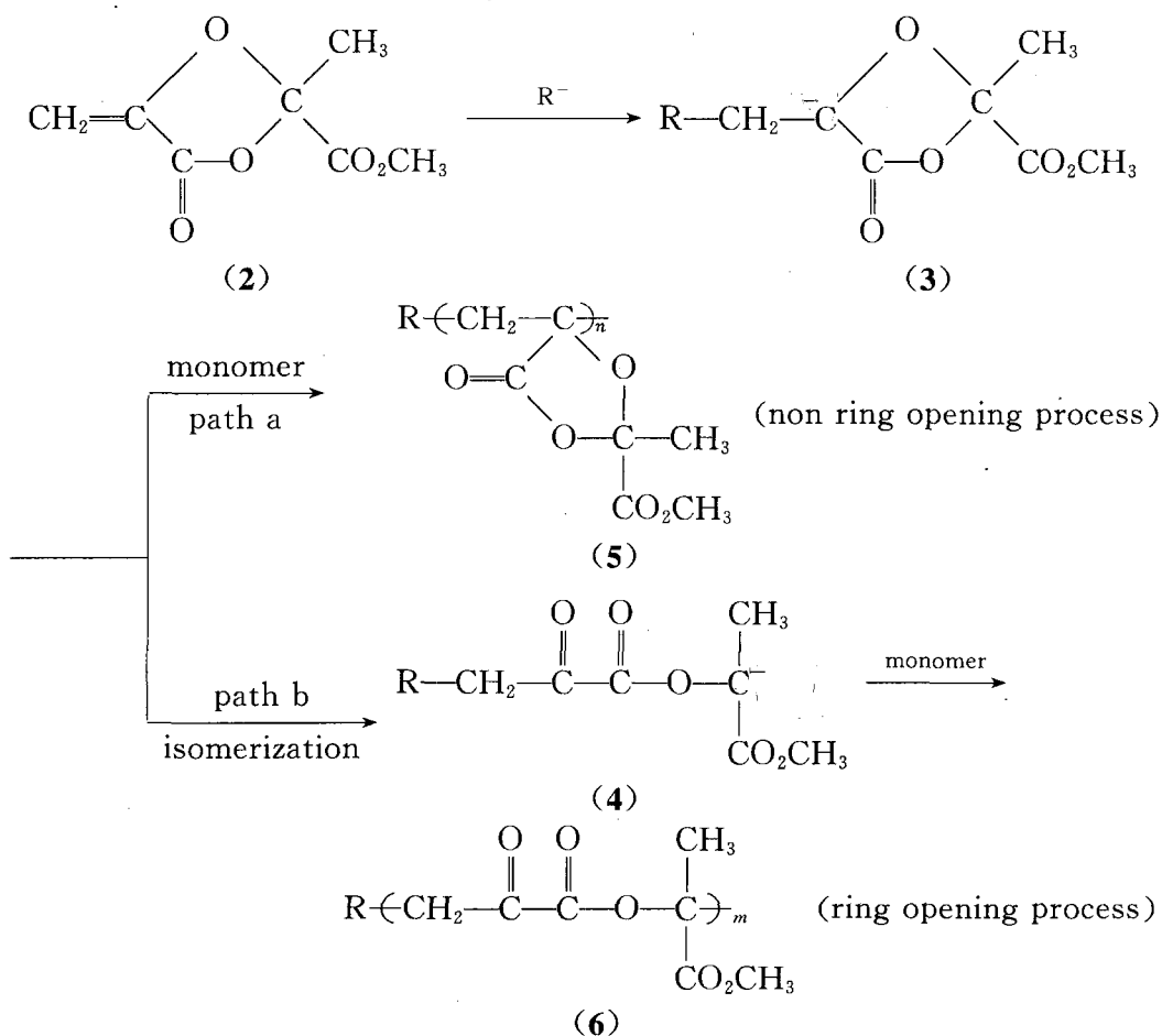
Scheme II Polymerization of the monomer
