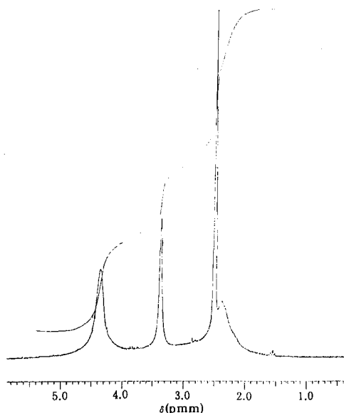
Fig. 1 ^1\text{H} NMR spectrum of the polymer in \text{DMSO-D}_6
